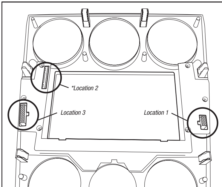
(99-7524 radio housing diagram)
