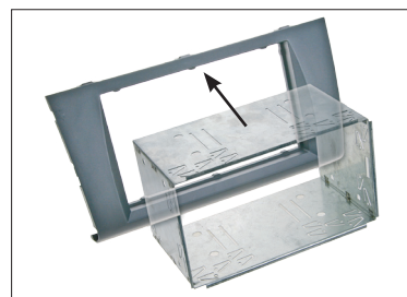
Place the Double-DIN fascia plate at the dashboard, move metal bracket into the fascia plate.
