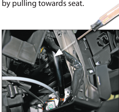
Remove locknut from head unit (driver's side underneath the dashboard). Place the screw driver BEHIND the frame as shown on the picture
