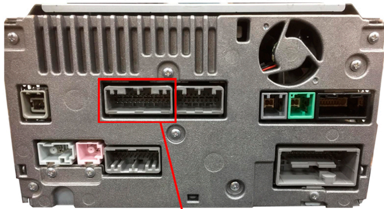
24 PIN CONNECTION
