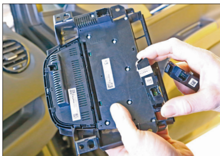
10. Remove switches and control unit from OEM panel
