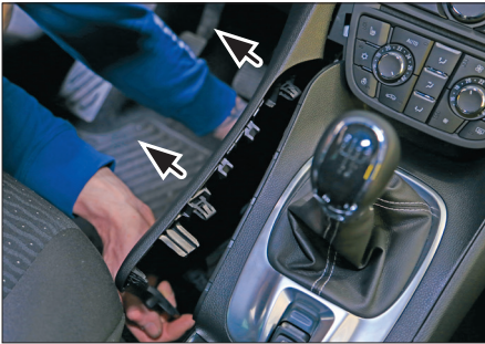
2. Unclip and remove side panels at the left and right side
