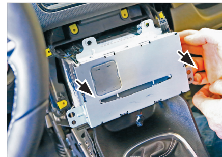
8. Unplug all cables and connectors carefully
