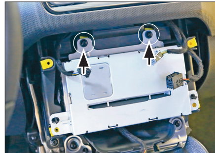
7. Remove two screws of OEM head unit
