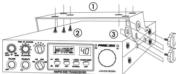
MOUNTING DIAGRAM
