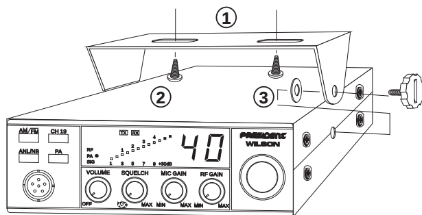
MOUNTING DIAGRAM
