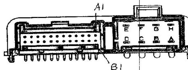
CONNECTOR DETAIL SCALE 2:1 ROTATED 90° CCW
