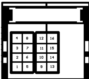
Vauxhall/Opel CAN-Bus
